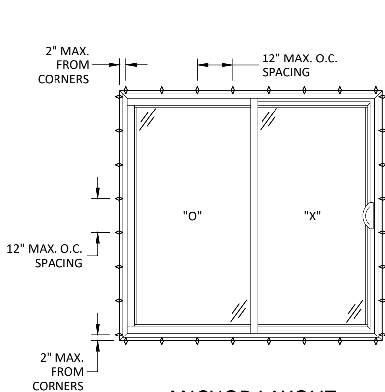
ANCHOR LAYOUT OX SLIDING GLASS DOOR 86.00" X 82.00" NAIL FIN INSTALLATION
