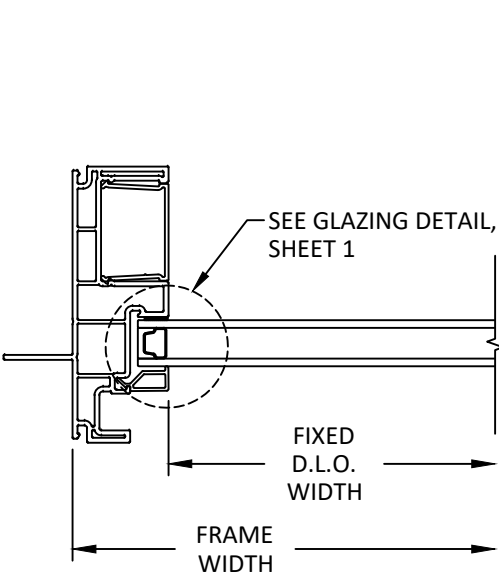
A 5 HORIZONTAL SECTION FIXED JAMB
